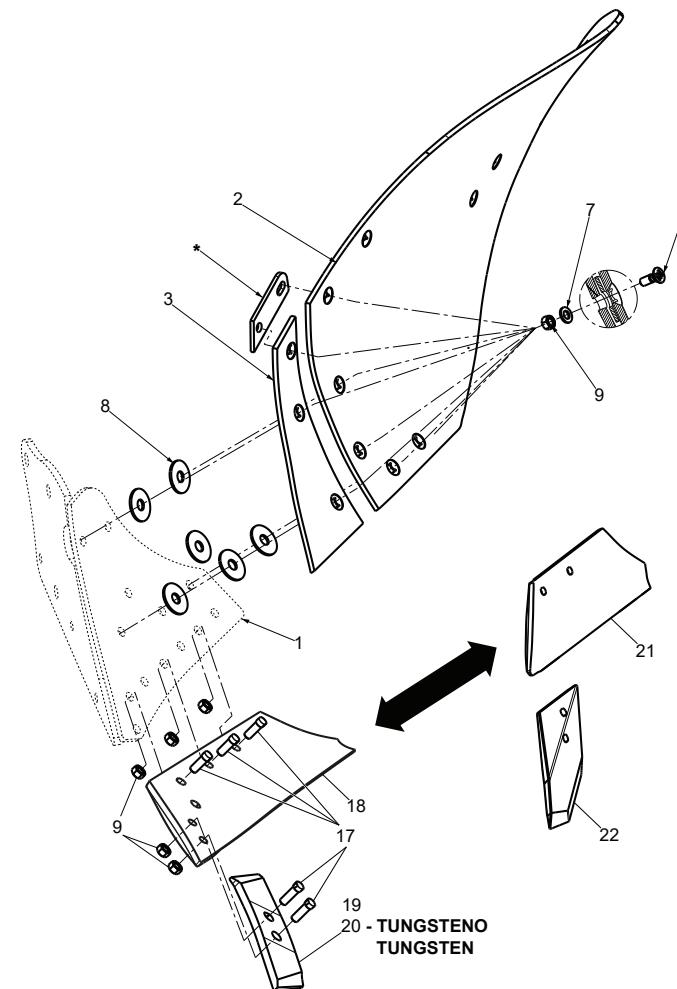
VISTA FRONTALE STANDARD STANDARD FRONT VIEW
