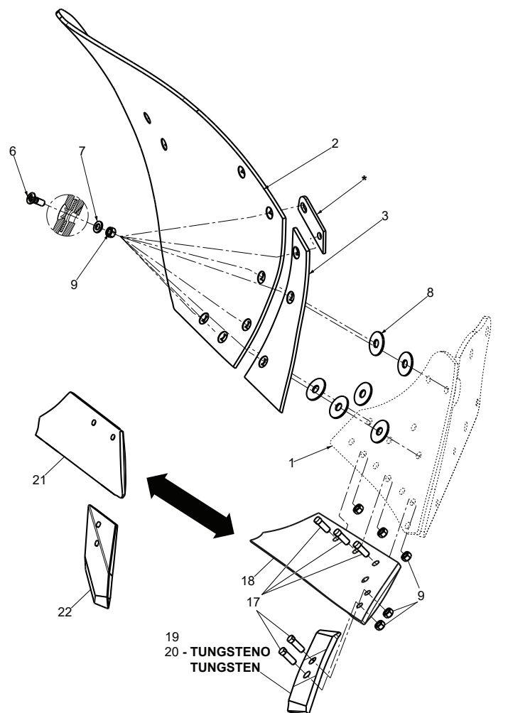
VISTA LATERALE STANDARD STANDARD SIDE VIEW
