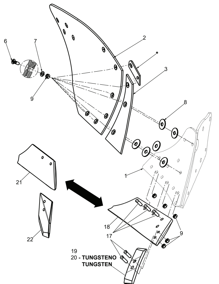
VISTA LATERALE STANDARD STANDARD SIDE VIEW
