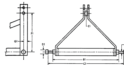
DIMENSIONS FOR REGULAR OR LIGHT DUTY IMPLEMENTS
