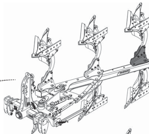
TRIVOMERE 3 WORKING ELEMENTS
